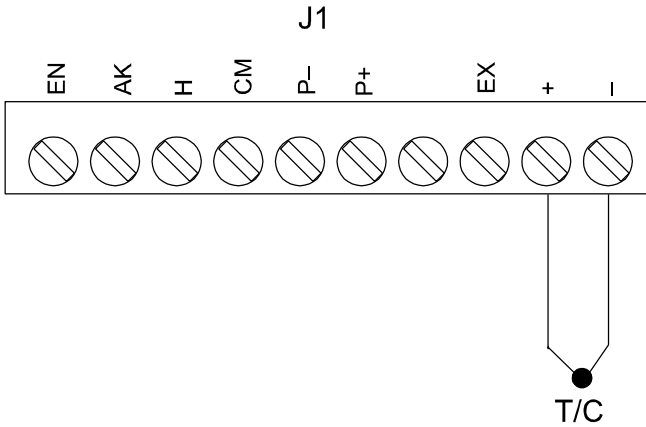
Figure 6. Thermocouple Connections
